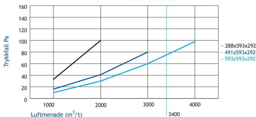
TRYKKFALLSDIAGRAM Viledon CarboPleat
