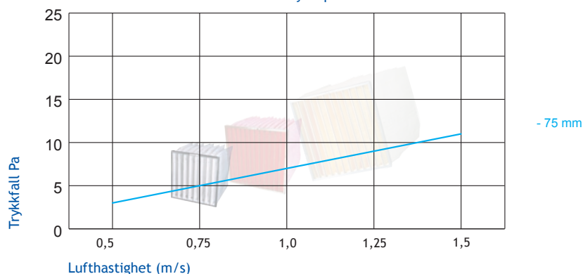
TRYKKFALLSDIAGRAM Hydropaint Collector
